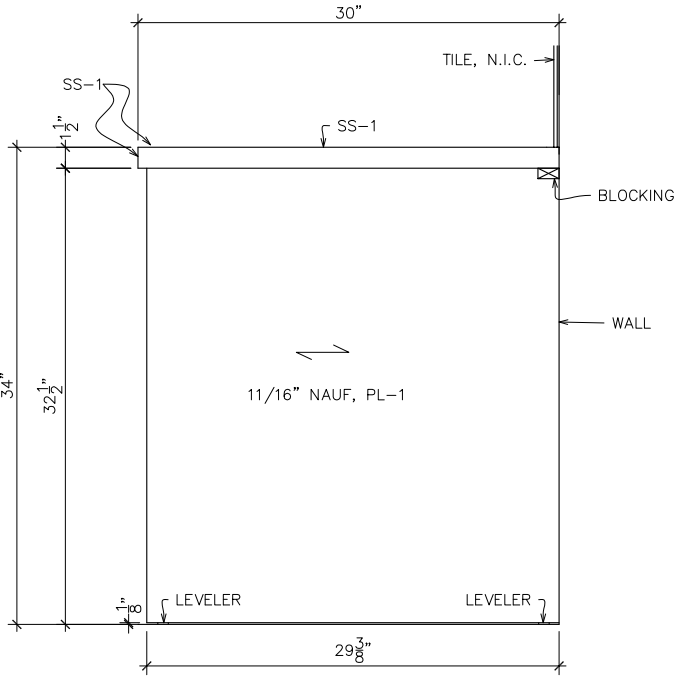
3 COUNTERTOP W/ SUPPORT 181.2 ARCH REF: 6A/A7.1
