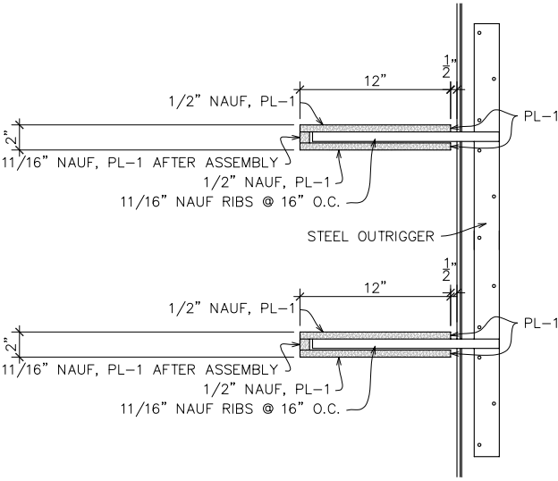
5 FLOATING SHELF SECTION 181.2 ARCH REF: 15A/ A7.1
