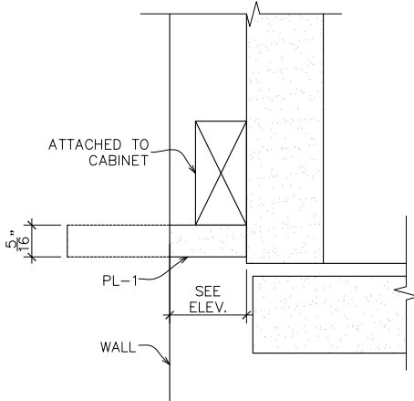
6 SCRIBE DETAIL 181.2 ARCH REF:
