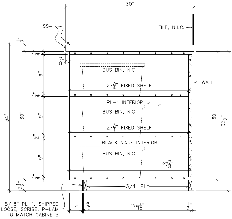
4 OPEN SHELF BASE SECTION 181.2 ARCH REF: 7A/A7.1
